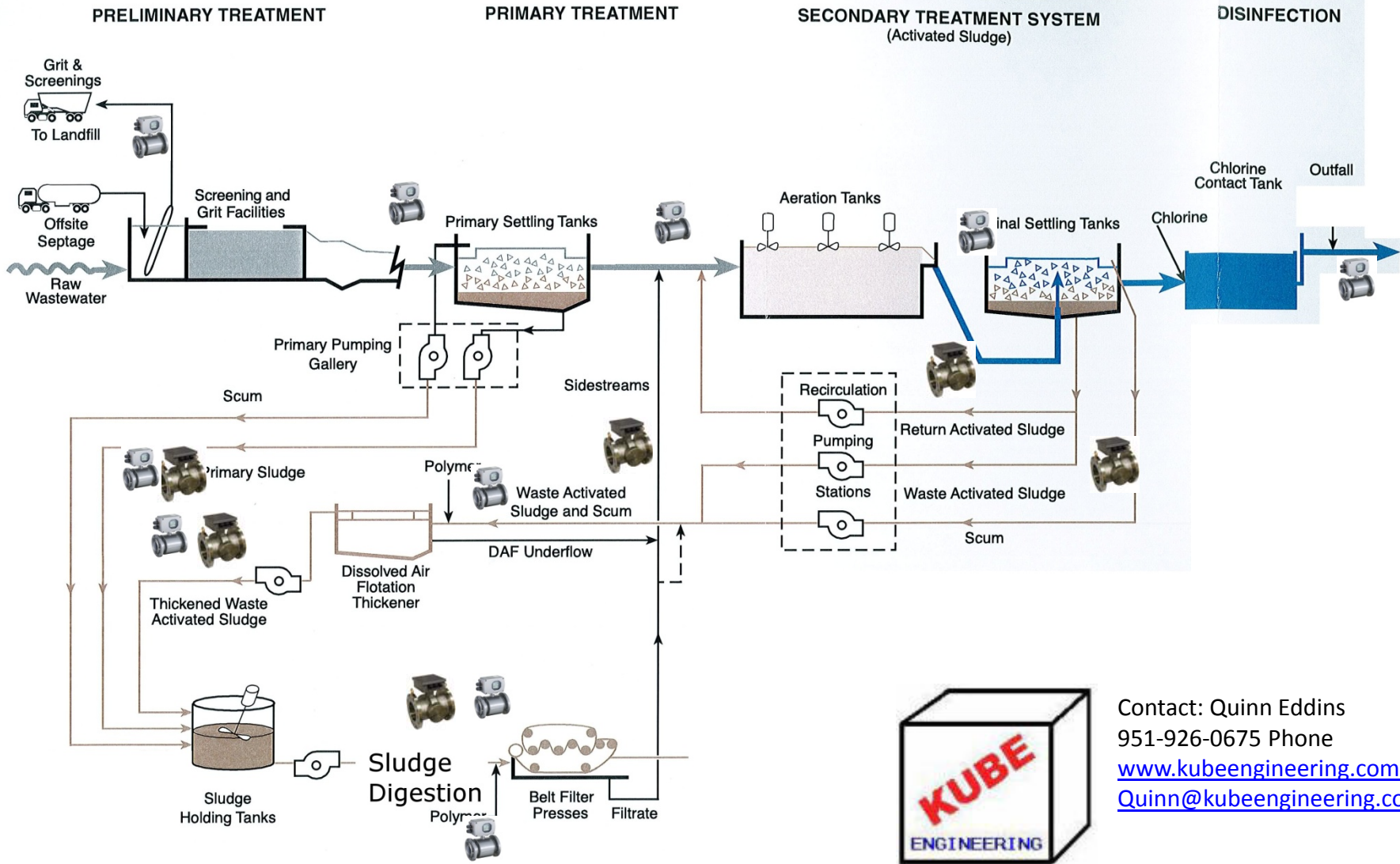
SLUDGE THICKENING AND DEWATERING
